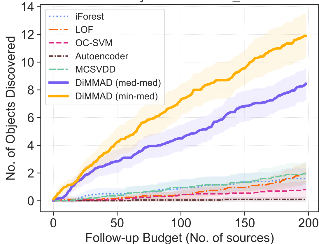
Anomaly: SNIn+HostXT_V19
